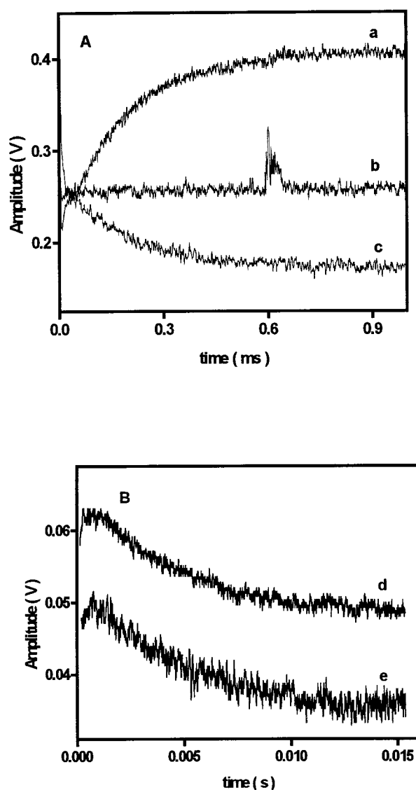
FIGURE 4 Effects of the transient electric field on the poly(A)-PR system (investigated with joule heating and absorbance detection). pH = 5.2, C_D = 3.0 \times 10^{-5} M, C_S/C_D = 3.33 , T = 25^\circ\text{C} . (A) I = 0.01 M, rise time = 1 \mu\text{s} , heating time = 49 \mu\text{s} . The traces have been recorded with different directions of the polarizer with respect to the transient electric field: (a) parallel, (b) magic angle ( 55^\circ ), (c) perpendicular. The wavelength is that of the isosbestic point (460 nm), where the effects of the chemical reaction are suppressed. (B) I = 0.1 M, rise time = 50 \mu\text{s} , heating time = 7.4 \mu\text{s} , \lambda = 430 nm. (d) No polarizer, \tau_1 = 0.41 ms and \tau_2 = 4.2 ms. (e) Magic angle ( 55^\circ ), \tau_1 = 0.38 ms and \tau_2 = 4.6 ms.
