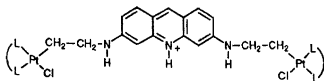
FIGURE 1 PRPt = [\{PtCl(tmen)\}_2\{HNC_{13}H_7(NHCH_2CH_2)_2\}]^+ . Tmen = L-L = N,N,N',N' -tetramethylethylenediamine.
