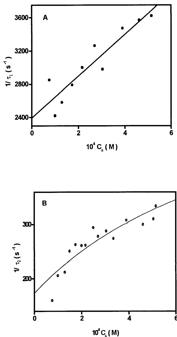
FIGURE 5 Reciprocal relaxation times as a function of the reactant concentrations for the poly(A)-PR system. pH = 5.2, I = 0.1 M, T = 25^\circ\text{C} . (A) Fast effect. (B) Slow effect.
